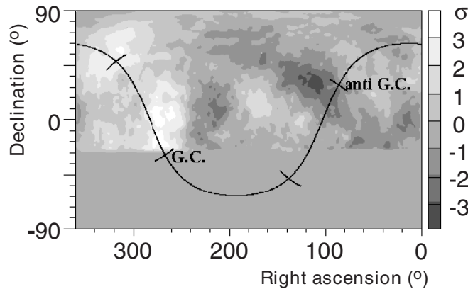
Figure 43. Significance map of anisotropy for EAS events between 8 \times 10^{17} and 2 \times 10^{18} eV in equatorial coordinates observed by AGASA [186]. Direction of galactic centre (GC) and anticentre (anti-GC) are shown. Events within a radius of 20^\circ are summed up in each bin.
