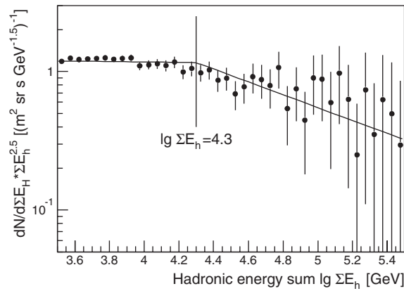
Figure 11. Flux spectrum of showers in the total hadronic energy measured by the KASCADE calorimeter. The observed knee is indicated by a vertical line (from [88]).
