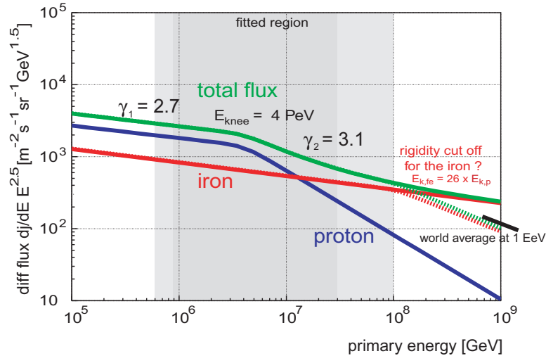
Figure 46. Motivation for the KASCADE-Grande experiment: Is there also a knee at the spectrum of the EAS induced by heavy primaries (from [36])?
