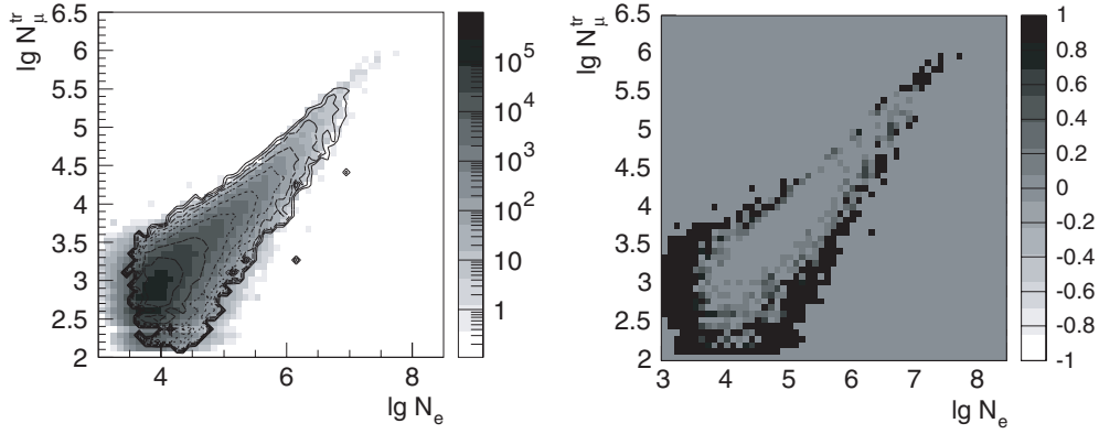
Figure 25. On the left-hand side the two-dimensional (N_e, N_\mu^{\text{tr}}) size spectrum (grey scale) measured by the KASCADE experiment is compared with the reconstructed distribution (contour). The corresponding difference (N_{\text{exp}} - N_{\text{MC}})/N_{\text{exp}} between experimental and simulated data is shown on the right-hand side [117]; \theta \in [0^\circ, 18^\circ] .
