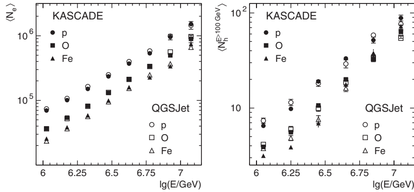
Figure 26. The projected relations \lg N_e and \lg N_h^{E>100 \text{ GeV}} , respectively, vs \lg(E/\text{GeV}) from a non-parametric analysis, trained to estimate the energy and mass of the measured events using N_e and N_\mu^E as EAS observables.
