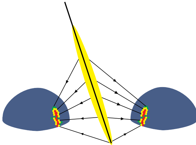
Figure 15. Schematic fluorescence detector assembly for stereo observation [101].
