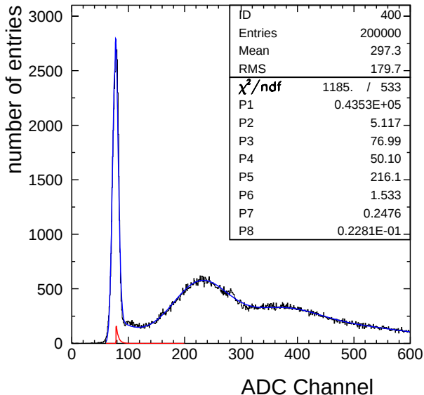
M16 ADC Spectrum at 1000V
