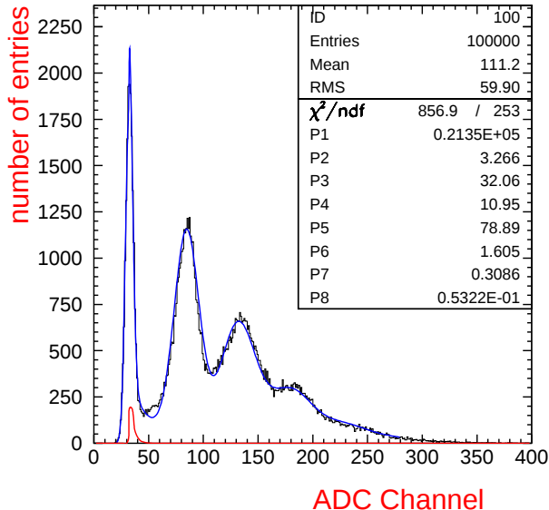
M64 ADC Spectrum at 1000V
