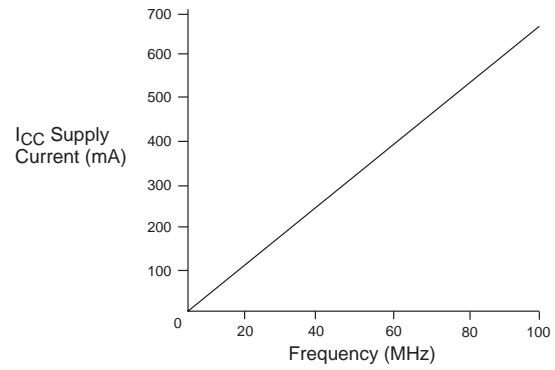
EPF10K50V
