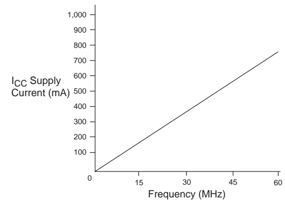
EPF10K40
