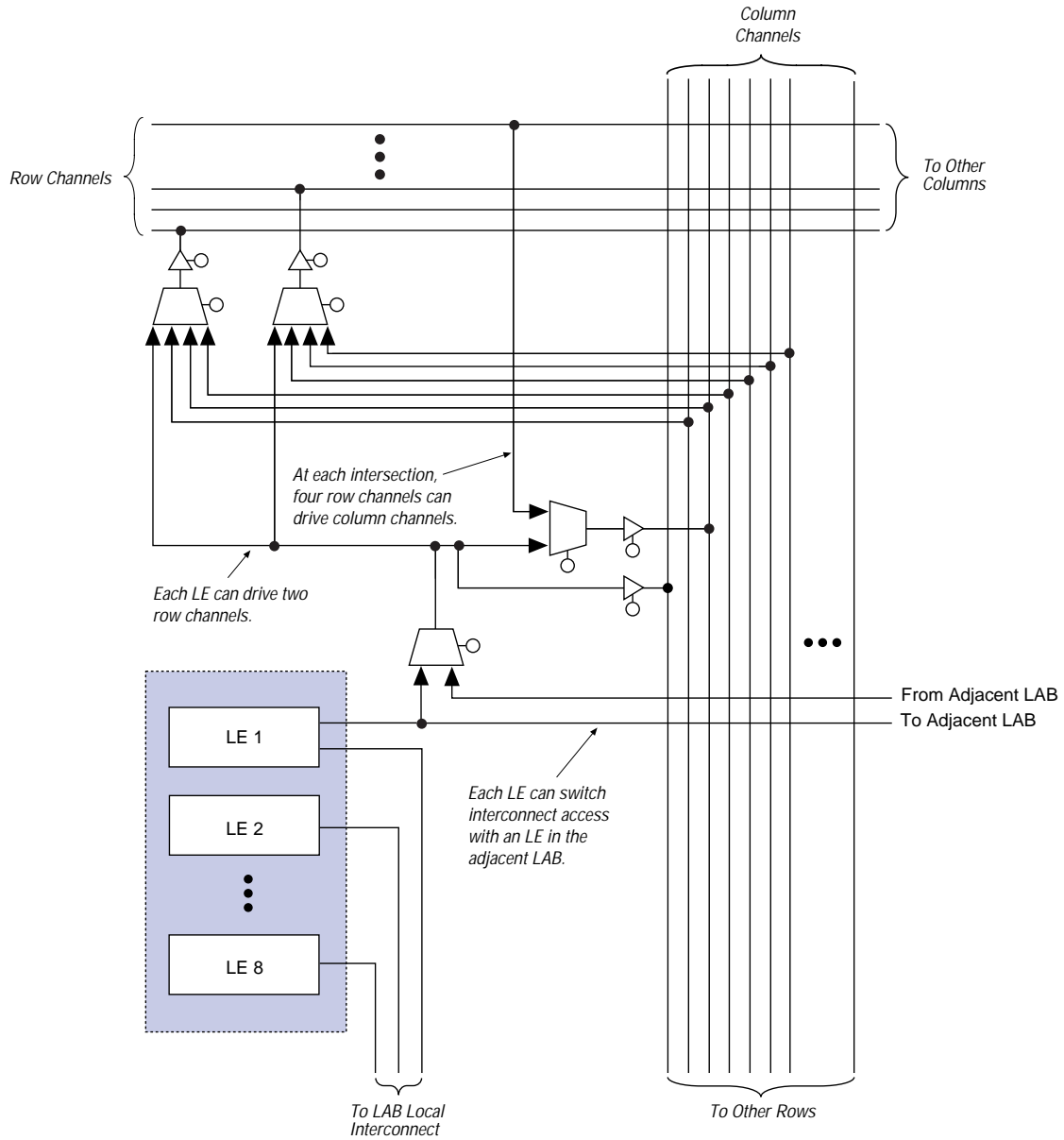
Figure 11. LAB Connections to Row &amp; Column Interconnect
