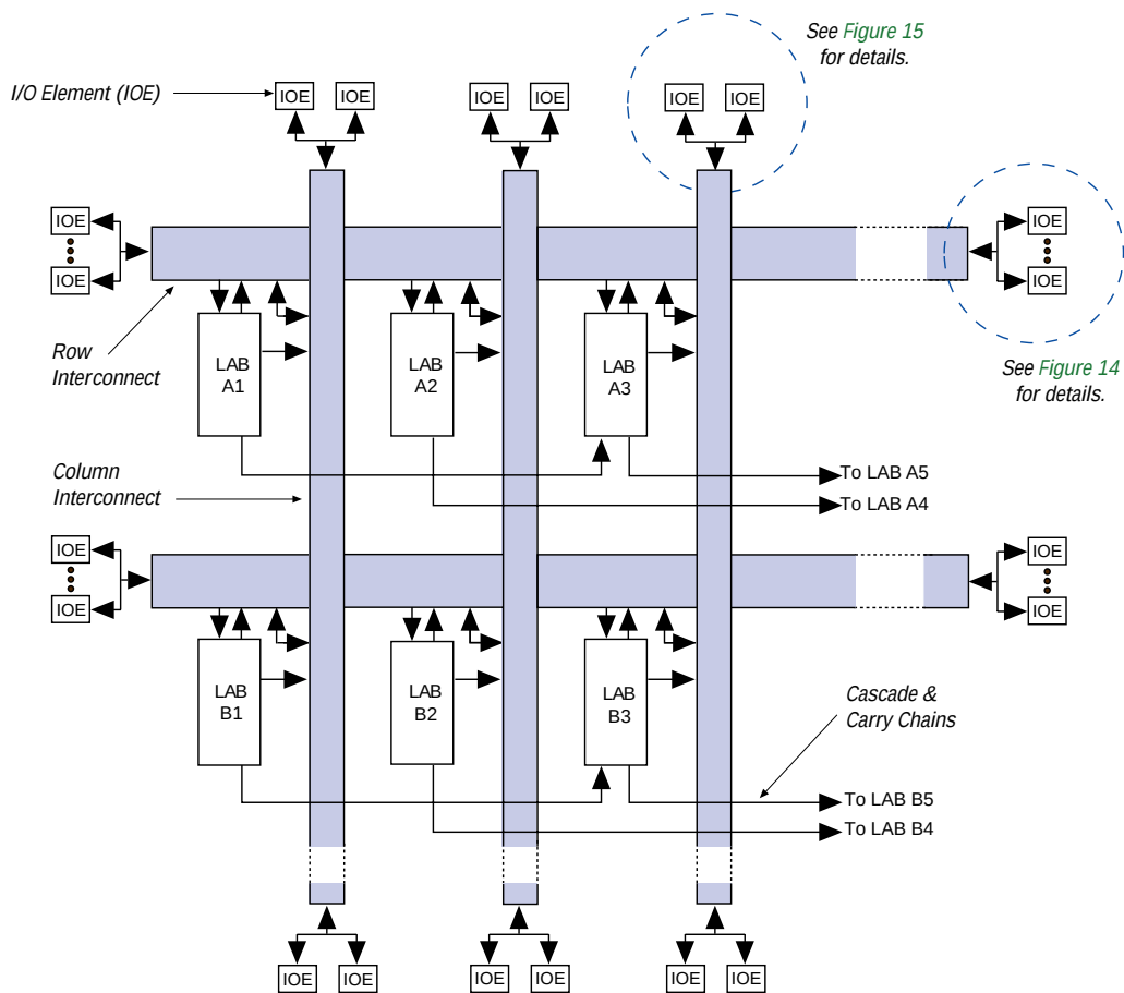
Figure 12. Interconnect Resources
