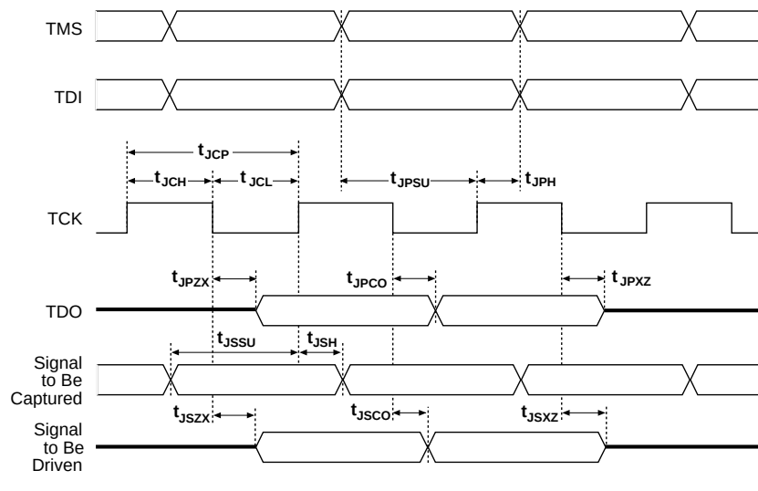
Figure 18. JTAG Waveforms
