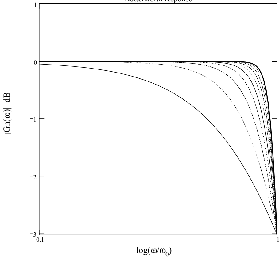
Butterworth response
