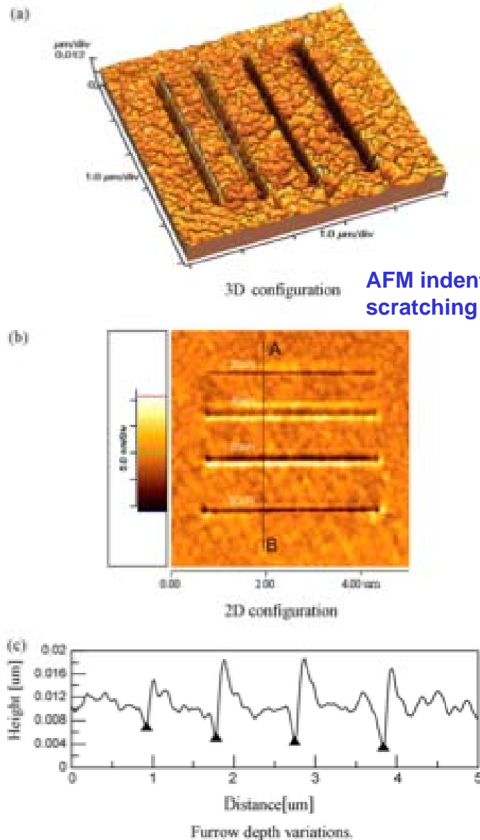
Fig. 1. The topographies of the line furrows for the loads of 20, 40, 60 and 80 μN. (a) 3D configuration, (b) 2D configuration, (c) furrow depth variations.
