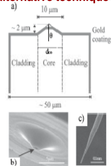
Figure 3.13: (a) Schematic of a SNOM fiber probe produced by selective chemical etching (SCE). The protruding cone is formed due to a slower etching rate of the core with respect to the cladding. After gold metallization (indicated by light gray lines), the tip is punched against a hard surface, producing a flattened apex with a sub-wavelength aperture at the center (black arrow), as evidenced by the SEM micrograph in (b).
