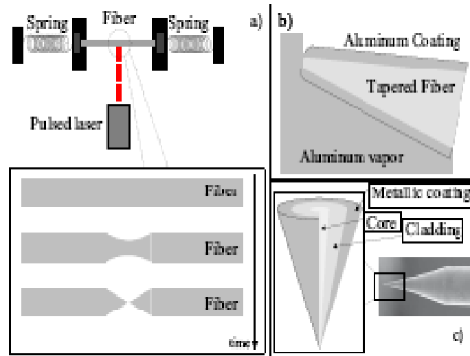
Figure 1.1: a) Heat and pull, one of the procedures to taper optical fibers for SNOM applications. b) Metallization of the SNOM fiber tip at a steep angle to leave a sub-wavelength aperture at the end. c) SEM image of the resulting tip and sketch of its interior.
