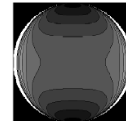
Fig. 3. Total electric field |\vec{E}|^2 in the aperture obtained by Bouwkamp.
