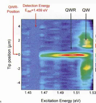
Fig. 7.24. Spatially resolved near-field photoluminescence excitation spectrum. The PLE signal is plotted as a function of tip position and excitation energy. The scan direction is perpendicular to the wire. The photoluminescence was detected at 1.46 eV. The color red corresponds to high and purple to low intensity.
